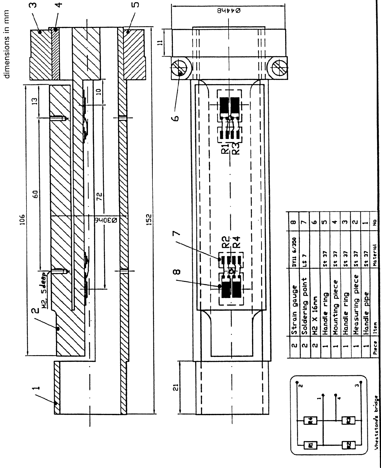
Figure B.1: Example of handle with gripping force measuring system
